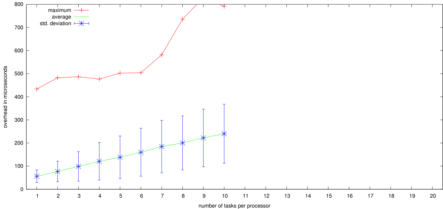
measured release interrupt overhead under G-EDF scheduling
