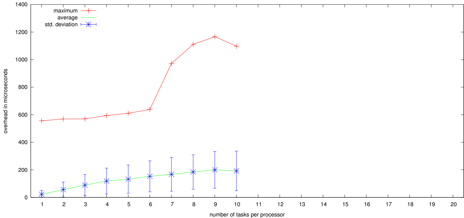
measured scheduling overhead under G-EDF scheduling
